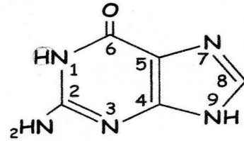
Guanine
